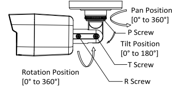
Figure 2-3 3-axis Adjustment
