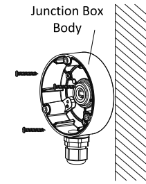
Figure 2-6 Fix the Junction Box to the Wall/Ceiling
