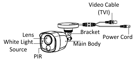
Figure 1-1 Camera Overview
