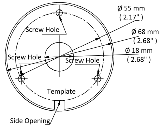
Figure 2-1 Drill Template
