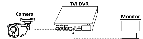
Figure 3-1 Connection
