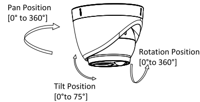
Figure 2-4 3-axis Adjusts
