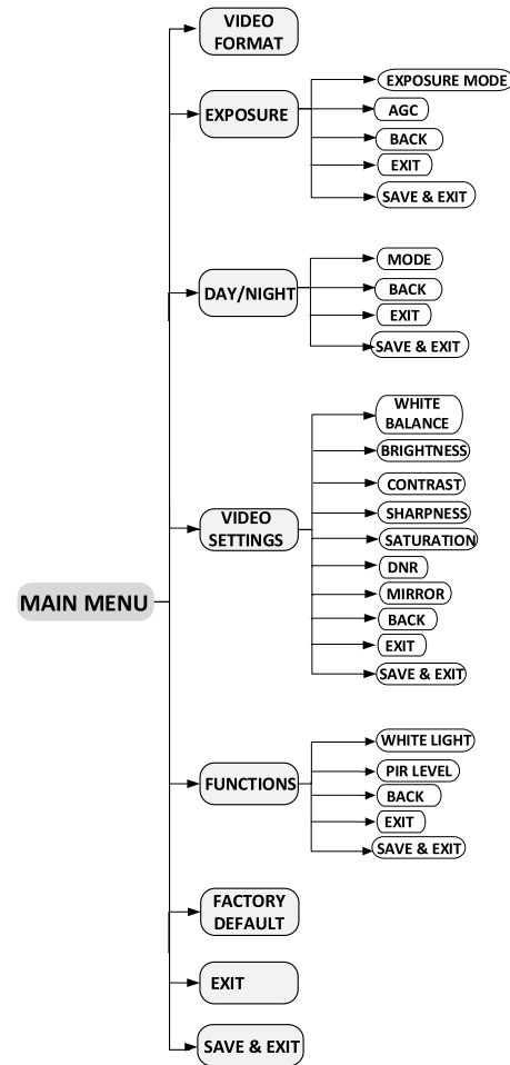
Figure 3-2 Main Menu Overview
