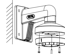
Figure 2-14 Install the Mounting Base to the Bracket
