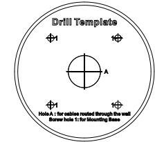
Figure 2-9 Drill Template of the Junction Box
