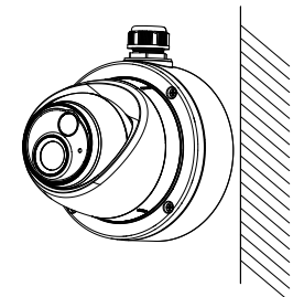
Figure 2-12 Fix the Camera to the Junction Box
