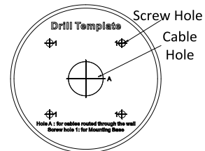
Figure 2-5 The Drill Template
