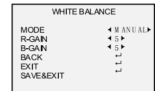
Figure 3-5 MWB MODE
